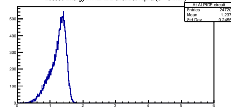
Lossed Energy in ALPIDE circuit at Alpha (d = 34mm)
